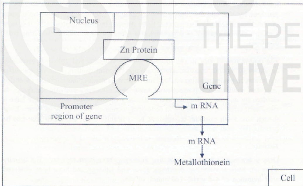
Figure 10.4: Interaction of transcription factor with zinc
