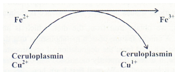
Figure 10.1: Oxidation of iron
