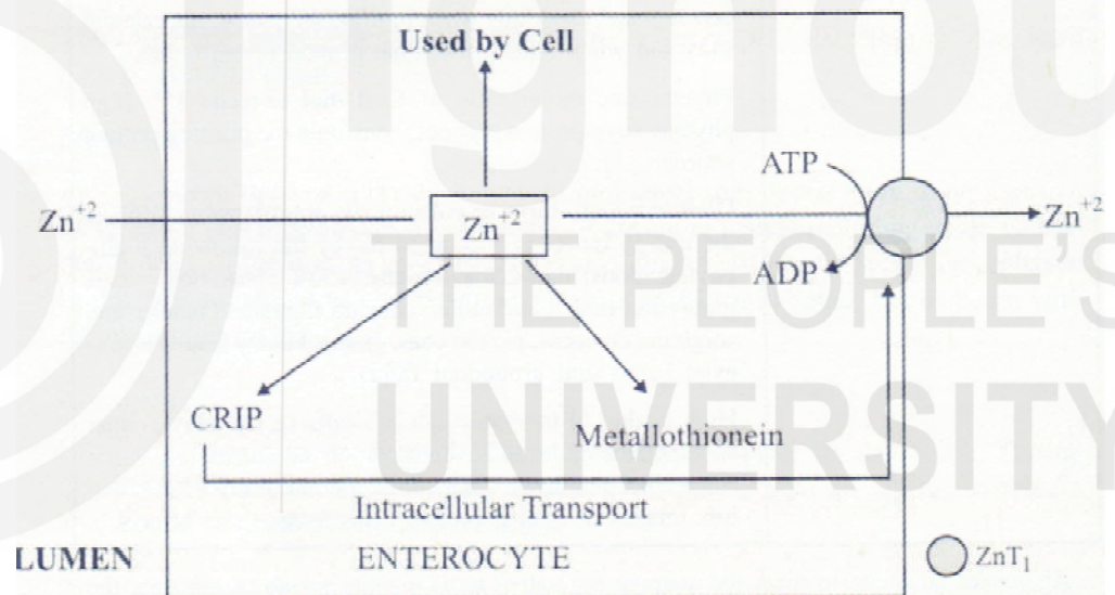
Figure 10.3: Enterocyte use and transport of zinc
