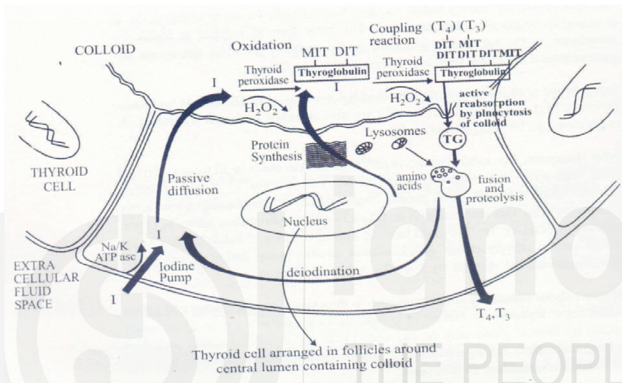
Figure 10.7: Biosynthesis and secretion of thyroid hormones
