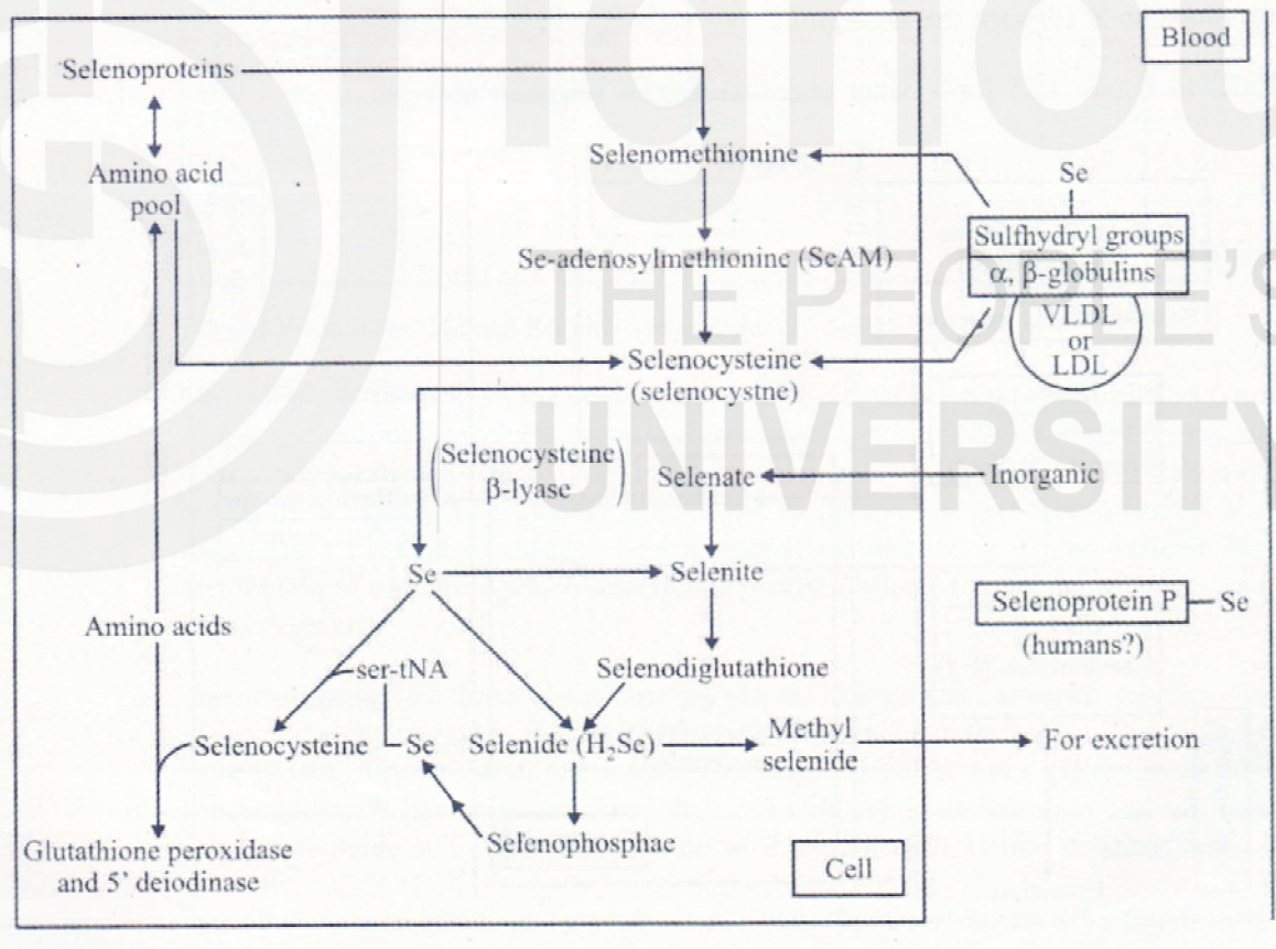
Figure 10.6: Metabolism of selenium in tissues
